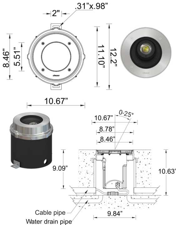
Mounting Detail
